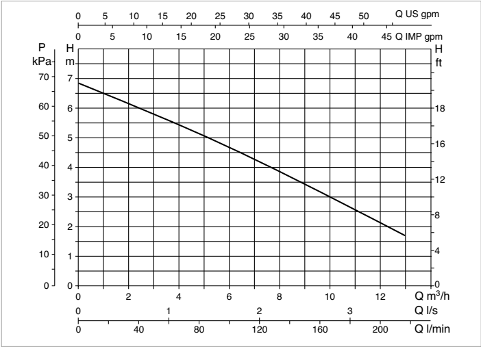
The performance curves are based on kinematic viscosity values = 1 mm²/s and density equal to 1000 kg/m³. Curve tolerance according to ISO 9906.
