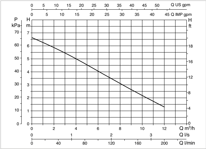
The performance curves are based on kinematic viscosity values = 1 mm²/s and density equal to 1000 kg/m³. Curve tolerance according to ISO 9906.
